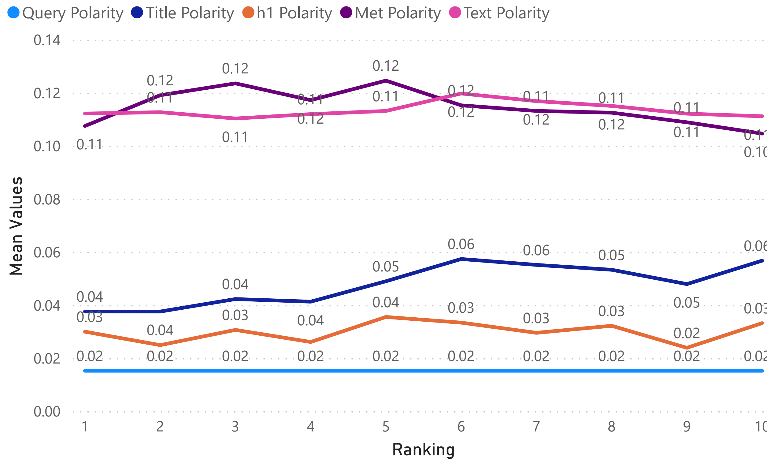
Mean Query Polarity, Title Polarity, h1 Polarity, Met Polarity and Text Polarity by Ranking
