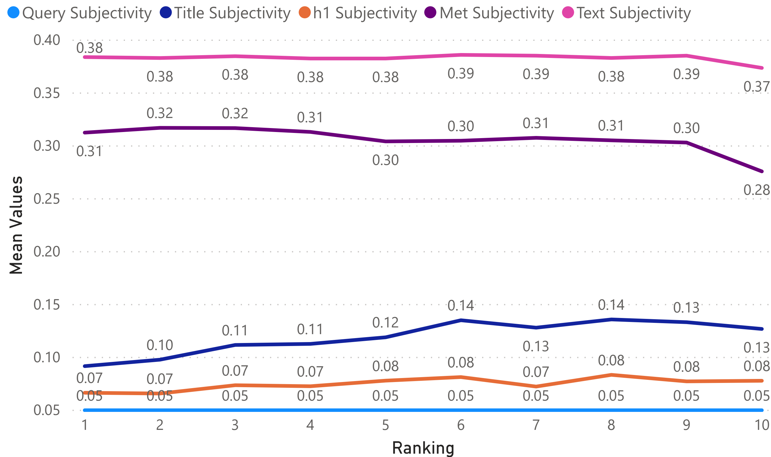
Mean Query Subjectivity, Title Subjectivity, h1 Subjectivity, Met Subjectivity and Text Subjectivity by Ranking
