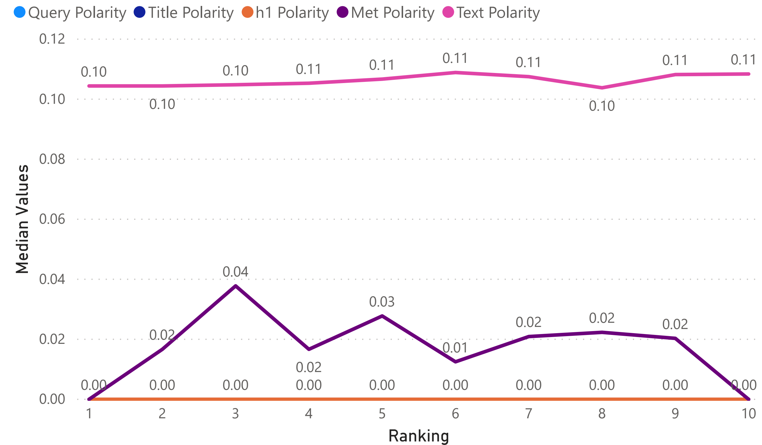
Median Query Polarity, Title Polarity, h1 Polarity, Met Polarity and Text Polarity by Ranking
