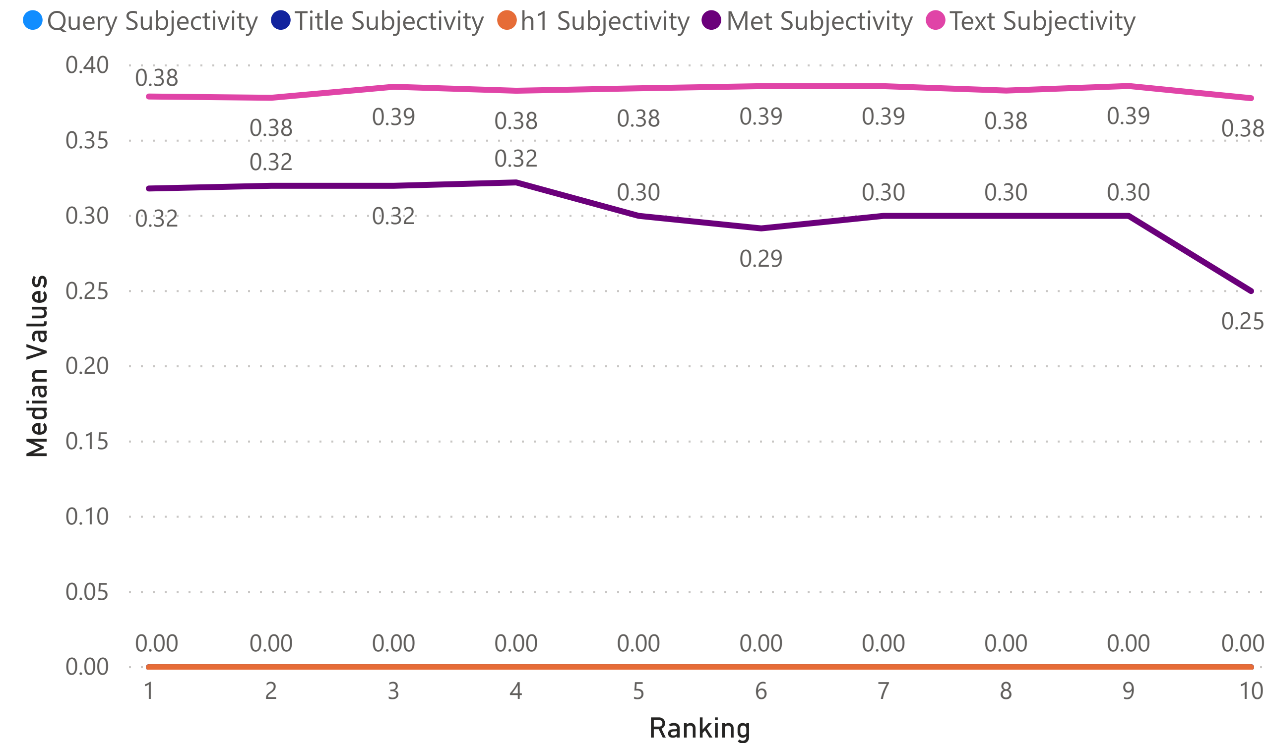
Median Query Subjectivity, Title Subjectivity, h1 Subjectivity, Met Subjectivity and Text Subjectivity by Ranking
